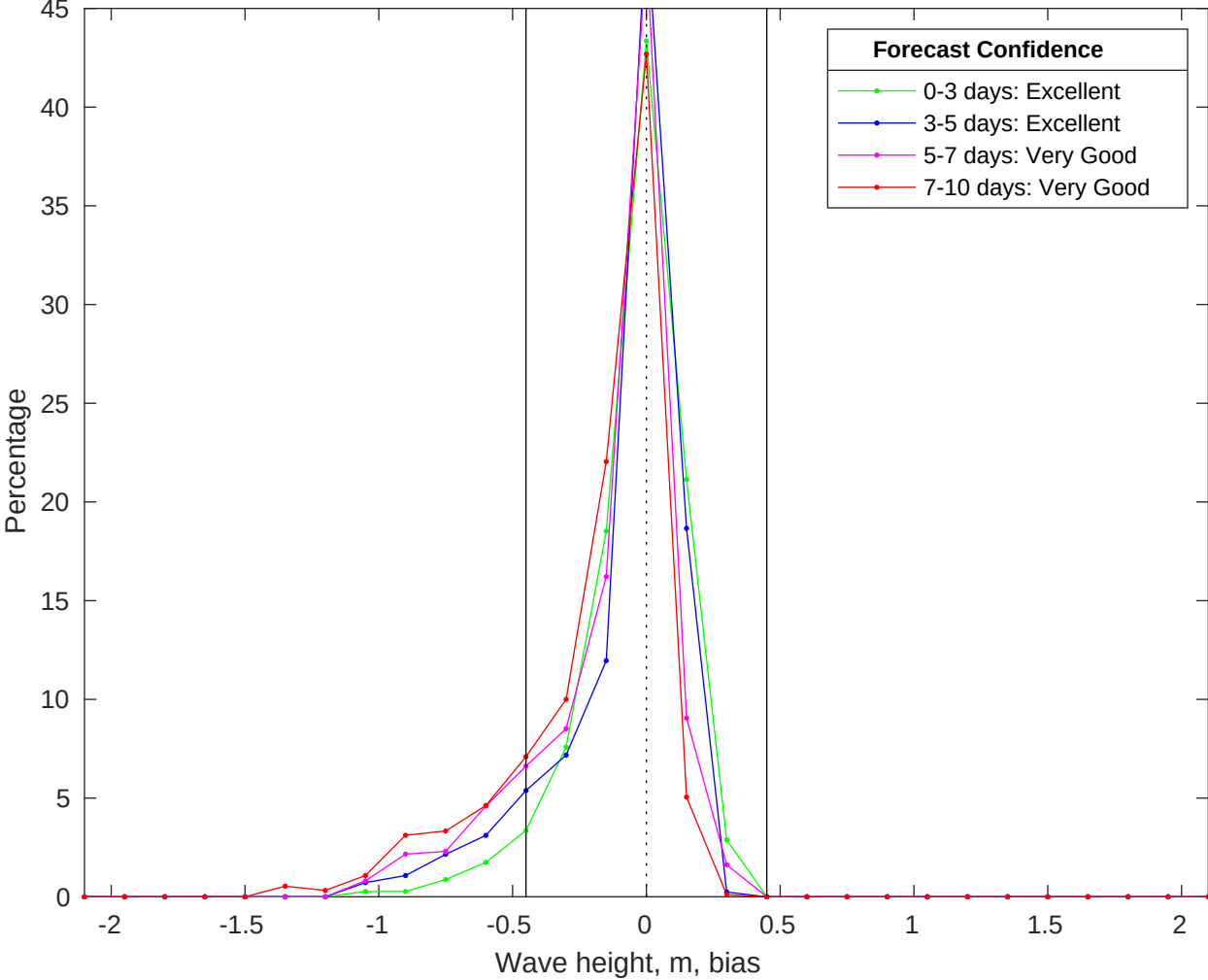
NDBC 52212 vs CMEMS Waves Bias Histogram: 15-Jun-2025
