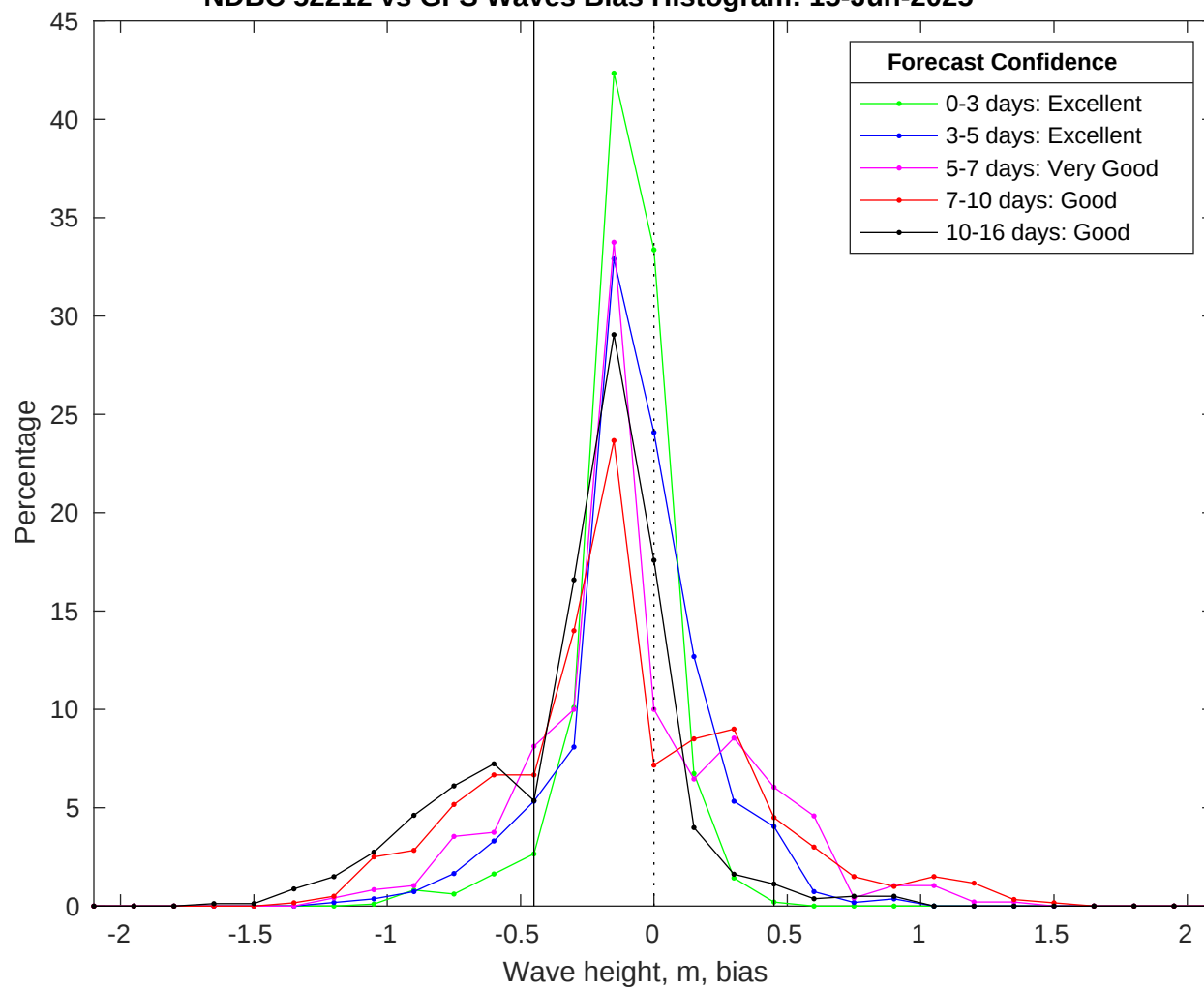
NDBC 52212 vs GFS Waves Bias Histogram: 15-Jun-2025
