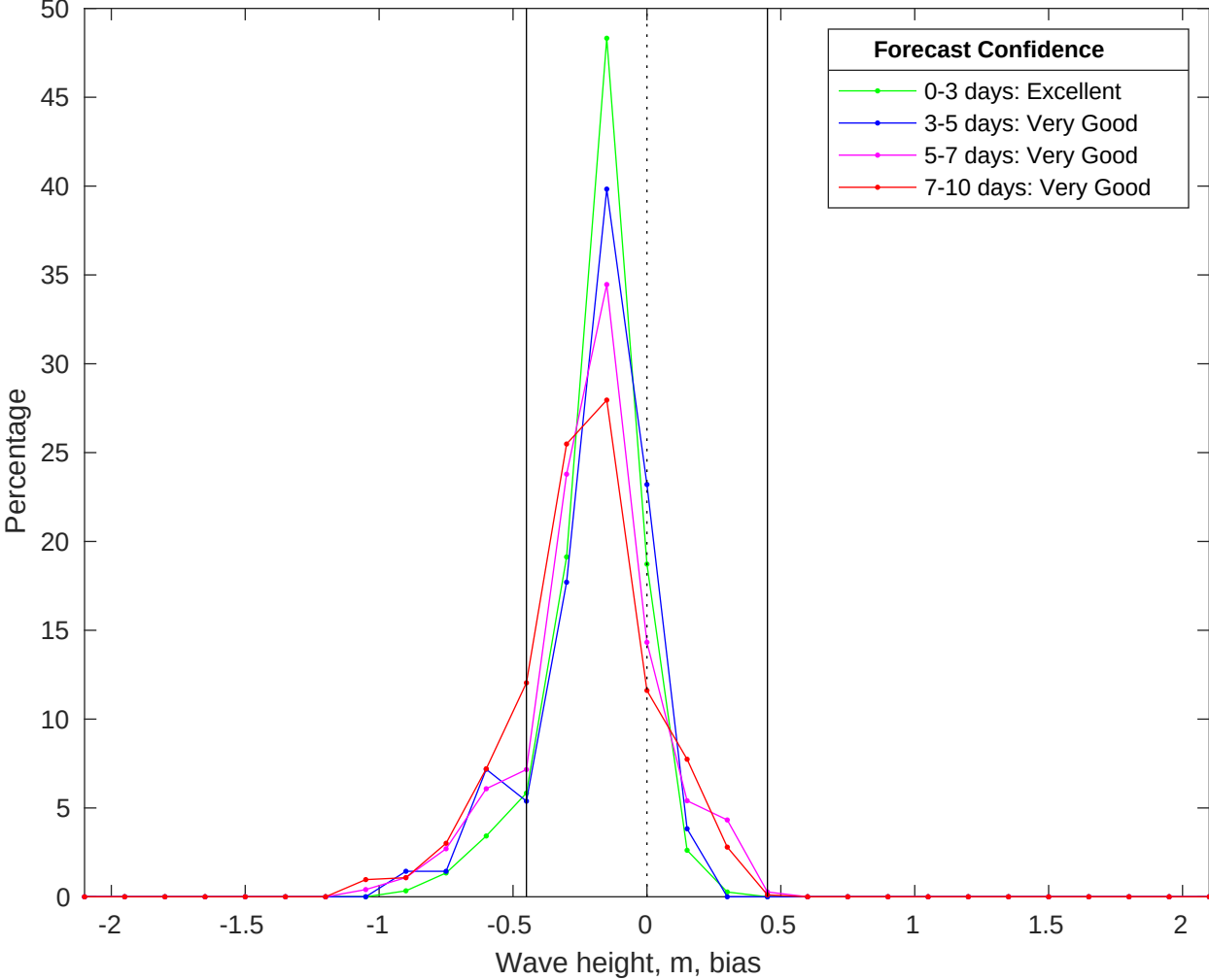
NDBC 52213 vs CMEMS Waves Bias Histogram: 15-Jun-2025
