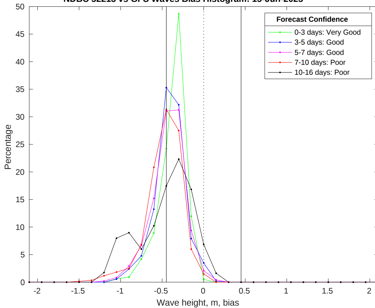
NDBC 52213 vs GFS Waves Bias Histogram: 15-Jun-2025
