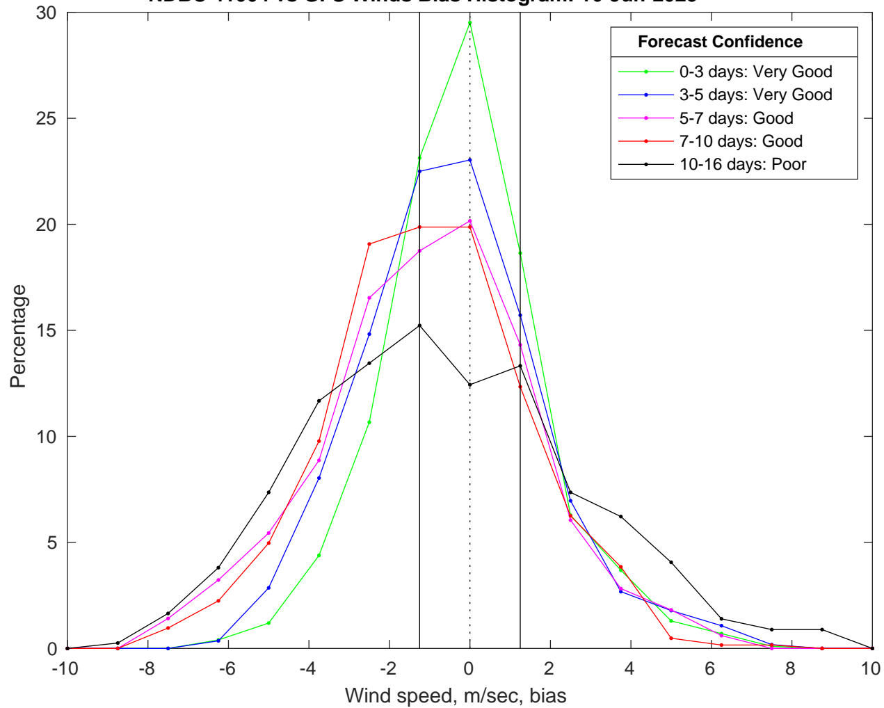
NDBC 41004 vs GFS Winds Bias Histogram: 16-Jun-2025
