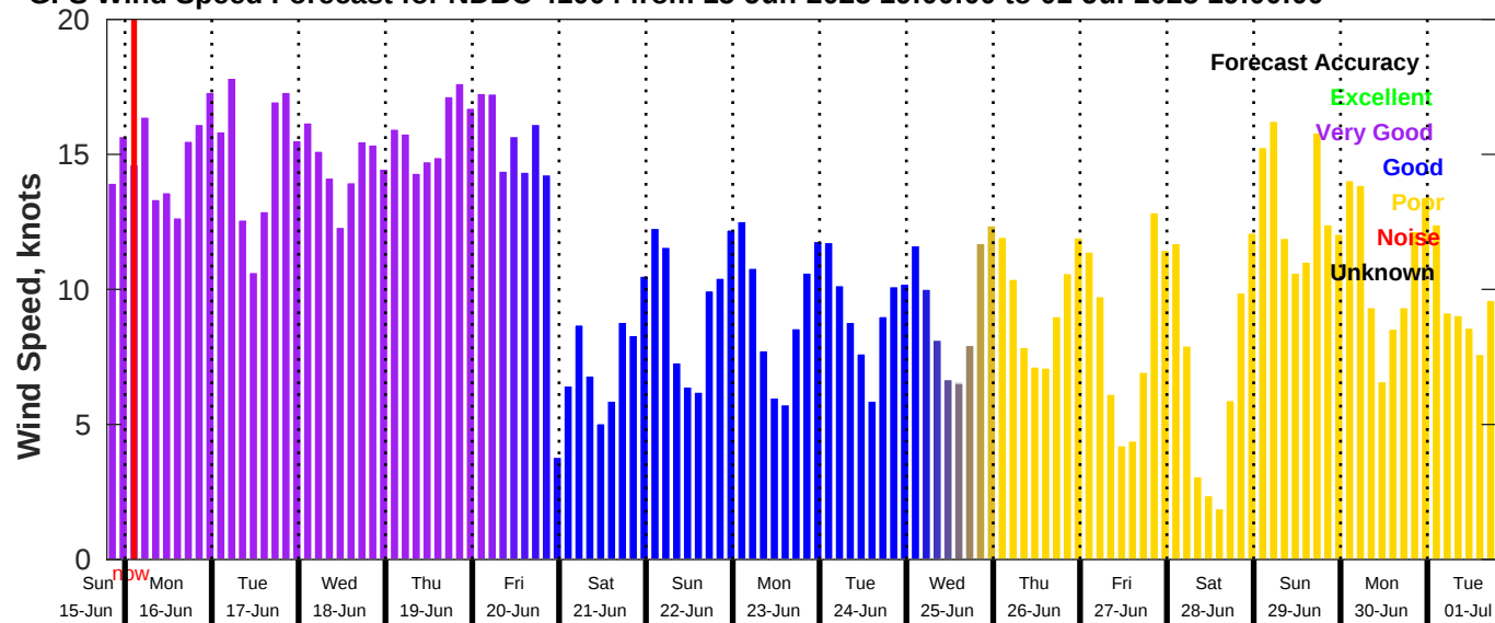
GFS Wind Speed Forecast for NDBC 41004 from 15-Jun-2025 19:00:00 to 01-Jul-2025 19:00:00
