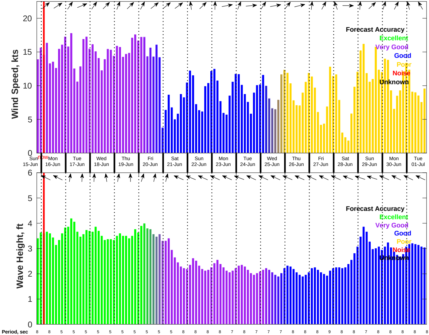
Wind & Wave Forecast for NDBC 41004 from 15-Jun-2025 19:00:00 to 01-Jul-2025 19:00:00
