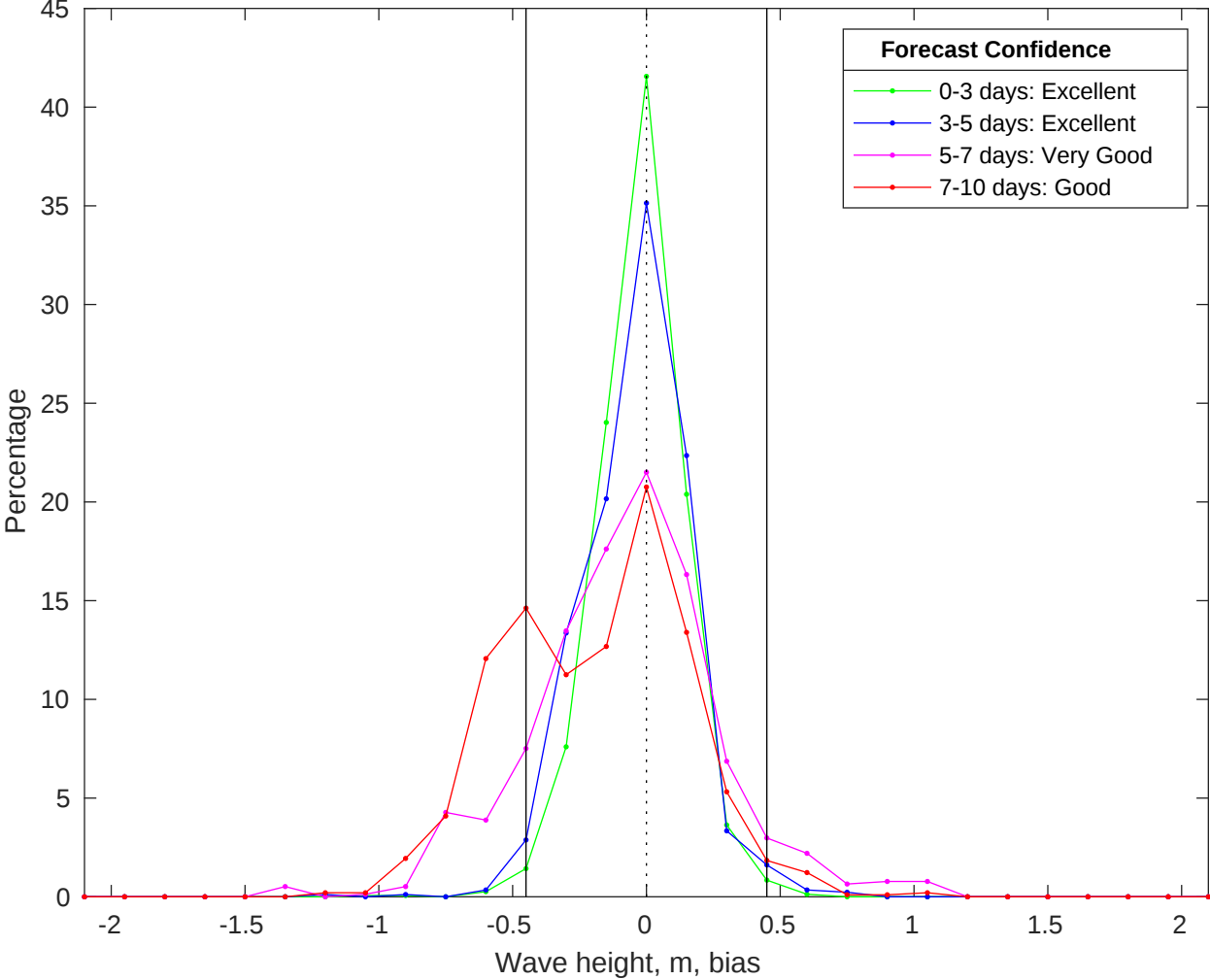
NDBC 41013 vs CMEMS Waves Bias Histogram: 16-Jun-2025
