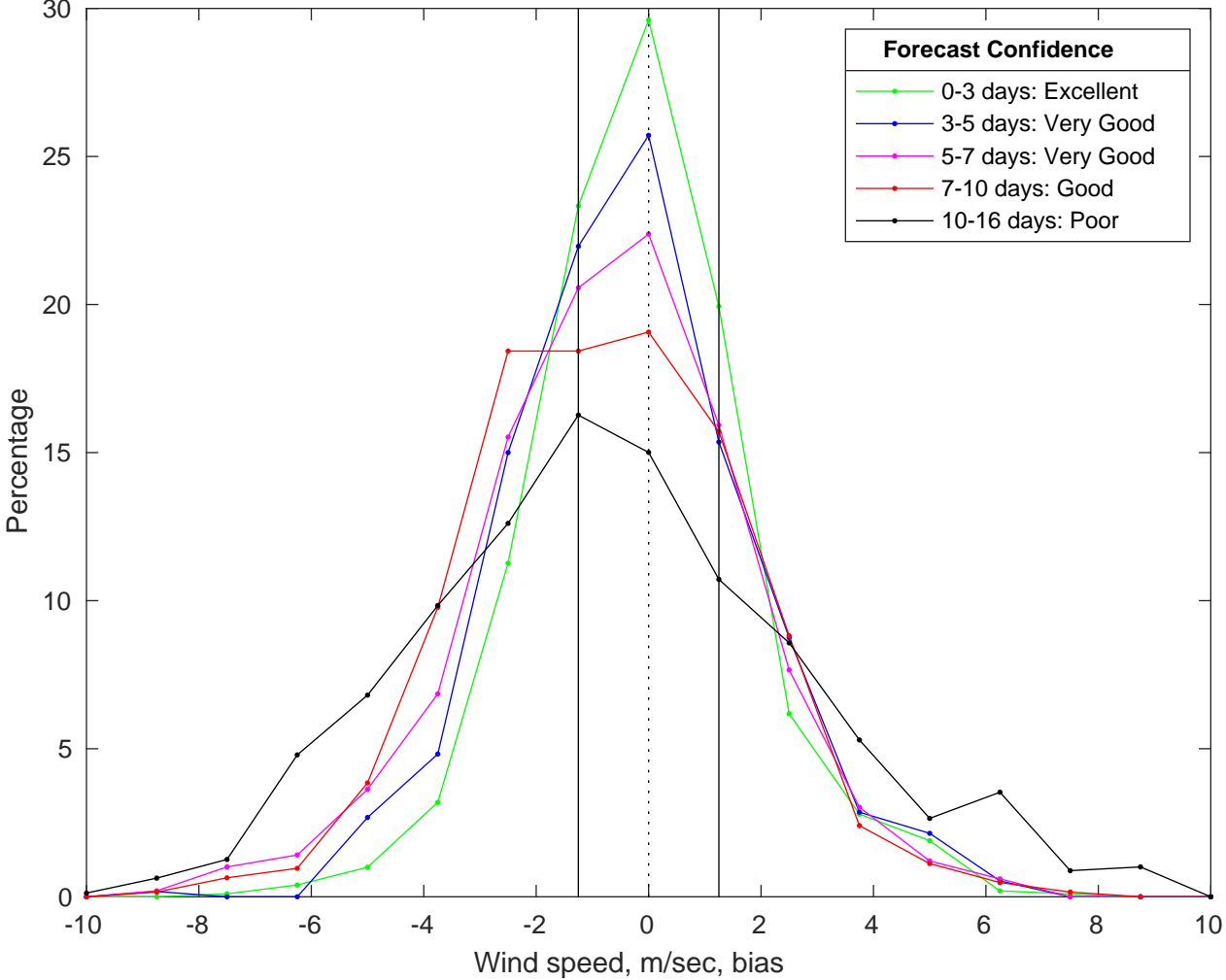
NDBC 41013 vs GFS Winds Bias Histogram: 16-Jun-2025
