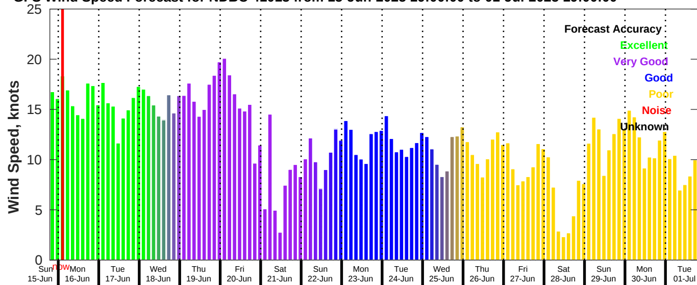
GFS Wind Speed Forecast for NDBC 41013 from 15-Jun-2025 19:00:00 to 01-Jul-2025 19:00:00
