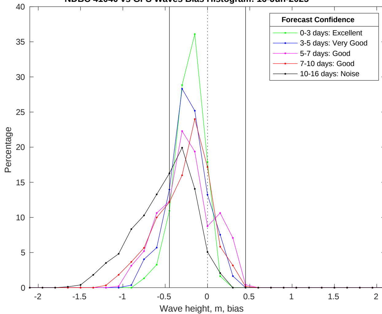
NDBC 41040 vs GFS Waves Bias Histogram: 16-Jun-2025
