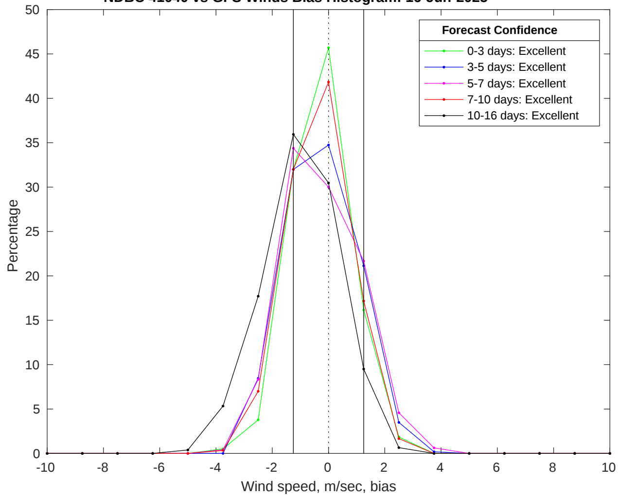
NDBC 41040 vs GFS Winds Bias Histogram: 16-Jun-2025
