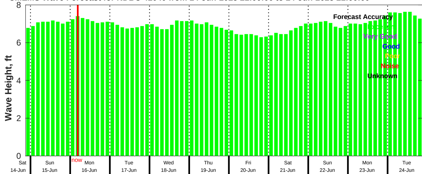
CMEMS Wave Forecast for NDBC 41040 from 14-Jun-2025 21:00:00 to 24-Jun-2025 21:00:00
