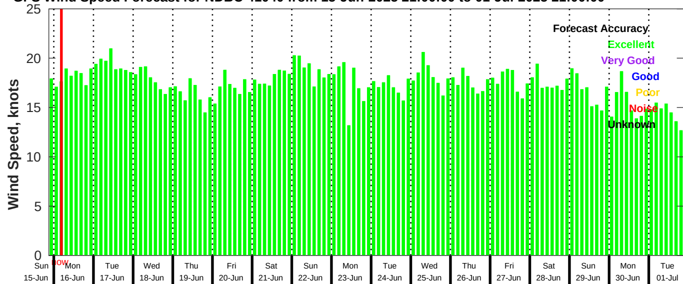
GFS Wind Speed Forecast for NDBC 41040 from 15-Jun-2025 21:00:00 to 01-Jul-2025 21:00:00
