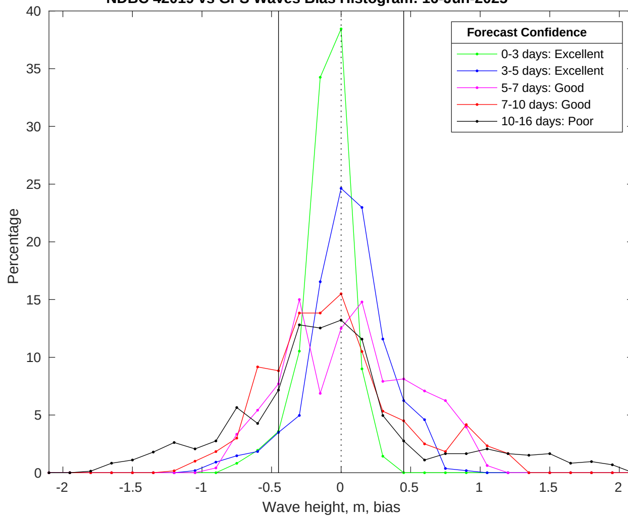
NDBC 42019 vs GFS Waves Bias Histogram: 16-Jun-2025
