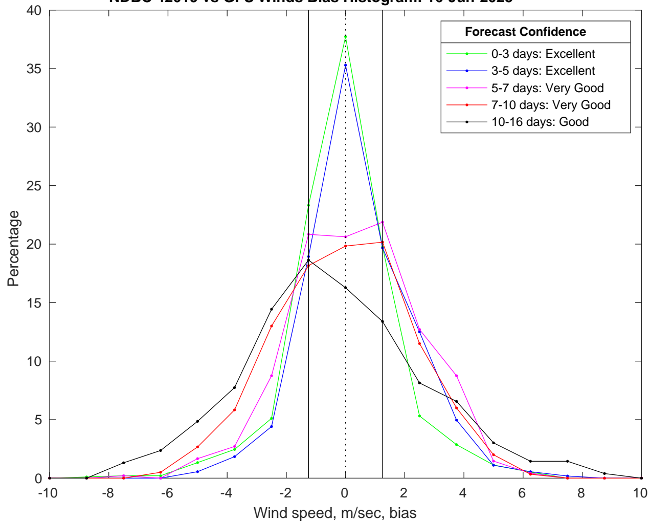
NDBC 42019 vs GFS Winds Bias Histogram: 16-Jun-2025
