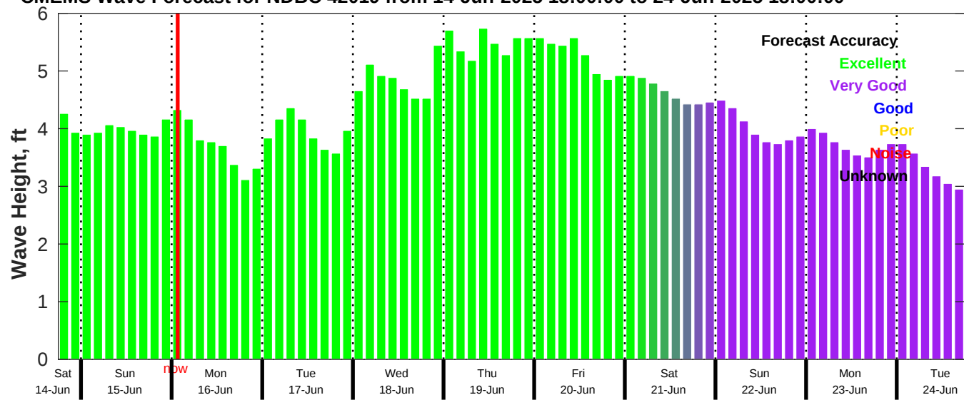
CMEMS Wave Forecast for NDBC 42019 from 14-Jun-2025 18:00:00 to 24-Jun-2025 18:00:00
