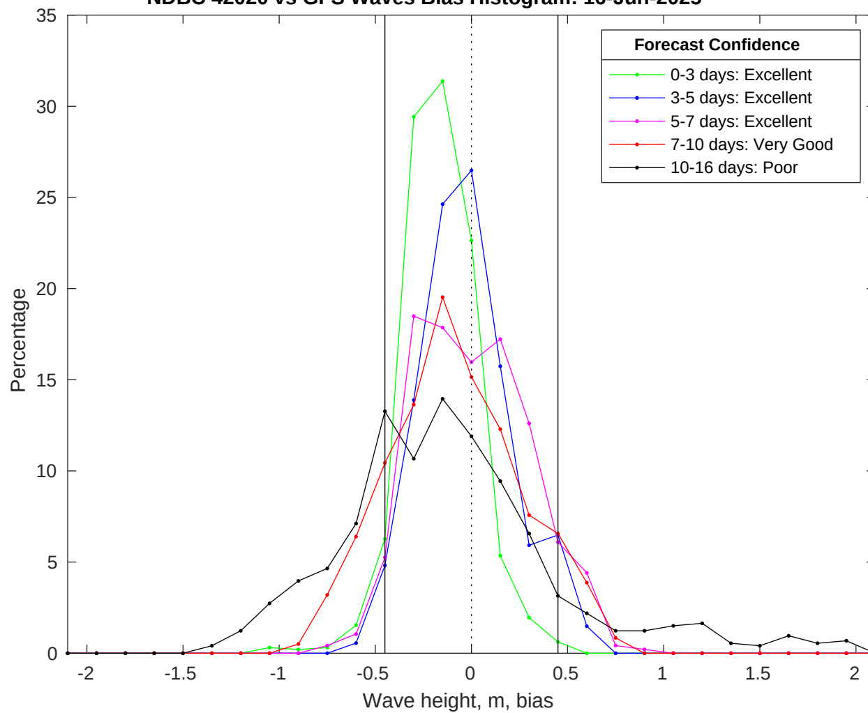
NDBC 42020 vs GFS Waves Bias Histogram: 16-Jun-2025
