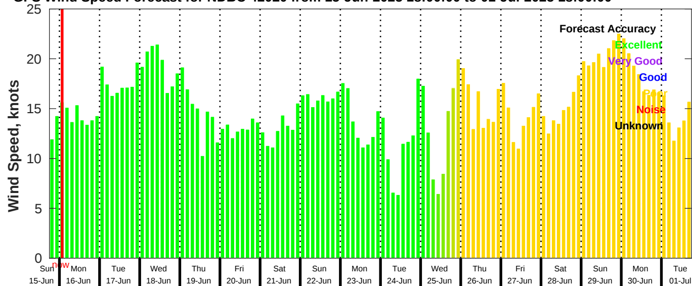
GFS Wind Speed Forecast for NDBC 42020 from 15-Jun-2025 18:00:00 to 01-Jul-2025 18:00:00
