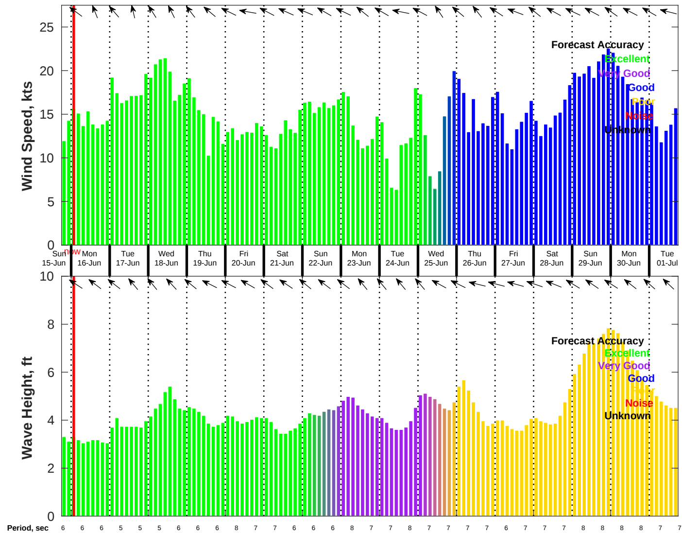
Wind & Wave Forecast for NDBC 42020 from 15-Jun-2025 18:00:00 to 01-Jul-2025 18:00:00
