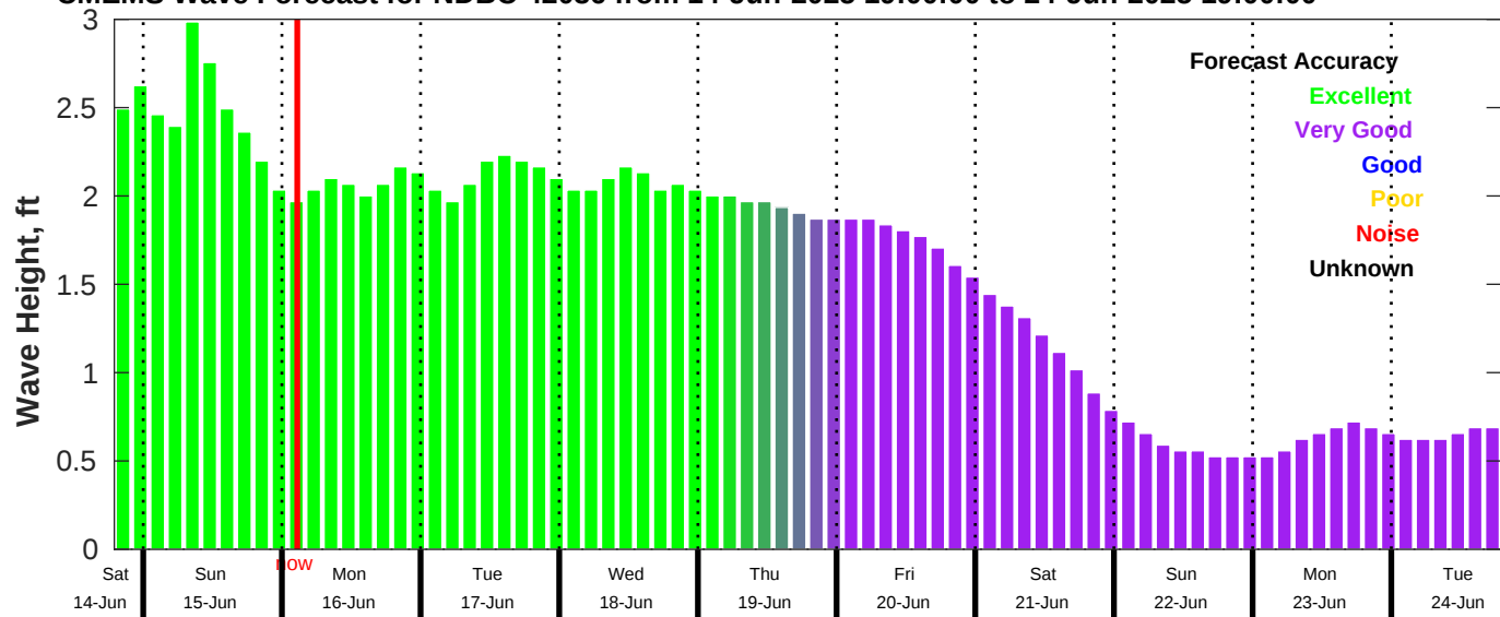
CMEMS Wave Forecast for NDBC 42036 from 14-Jun-2025 19:00:00 to 24-Jun-2025 19:00:00
