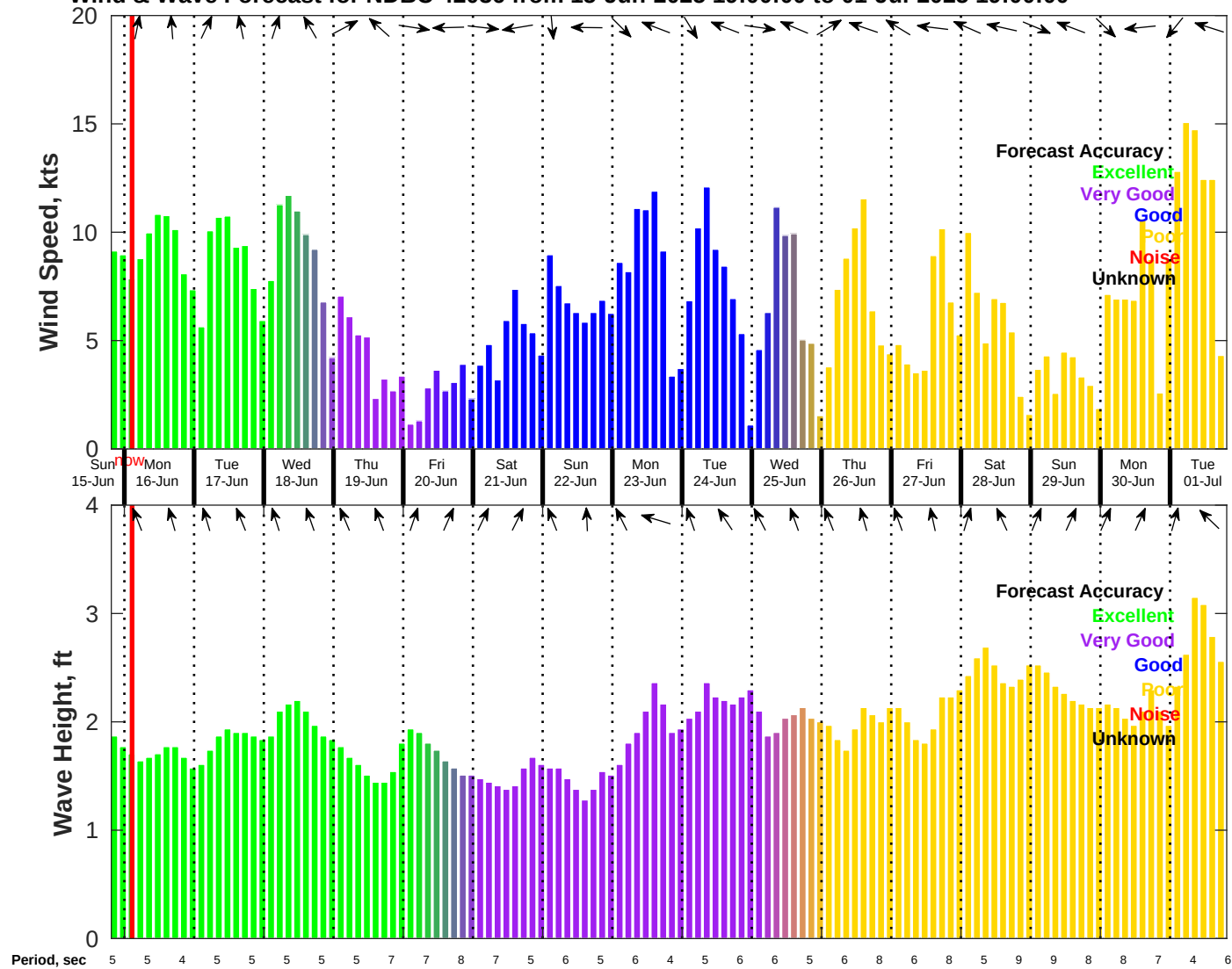
Wind & Wave Forecast for NDBC 42036 from 15-Jun-2025 19:00:00 to 01-Jul-2025 19:00:00
