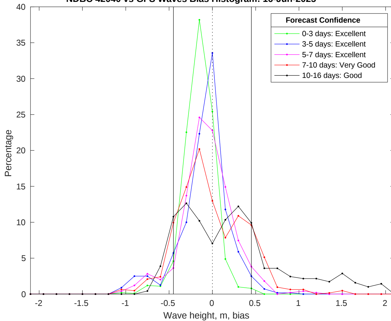
NDBC 42040 vs GFS Waves Bias Histogram: 16-Jun-2025
