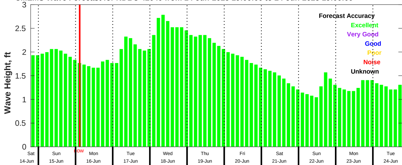
CMEMS Wave Forecast for NDBC 42040 from 14-Jun-2025 19:00:00 to 24-Jun-2025 19:00:00
