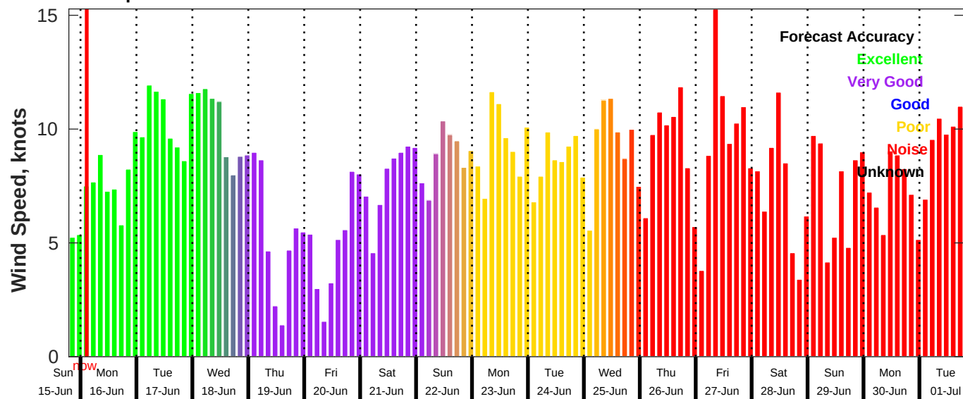
GFS Wind Speed Forecast for NDBC 42040 from 15-Jun-2025 19:00:00 to 01-Jul-2025 19:00:00
