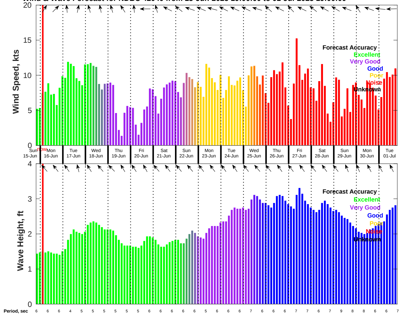
Wind & Wave Forecast for NDBC 42040 from 15-Jun-2025 19:00:00 to 01-Jul-2025 19:00:00
