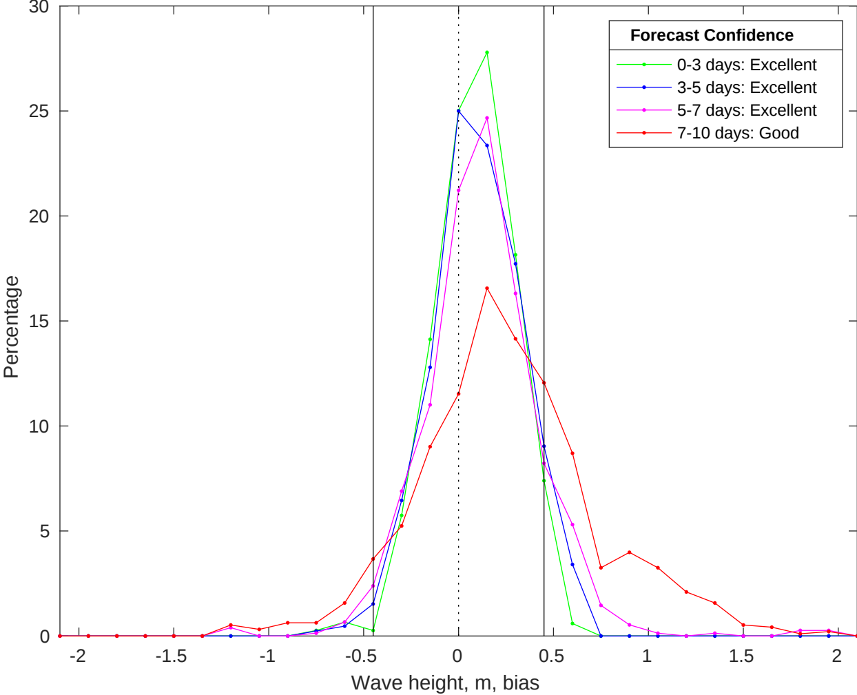
NDBC 46011 vs CMEMS Waves Bias Histogram: 16-Jun-2025
