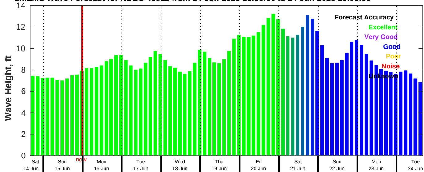
CMEMS Wave Forecast for NDBC 46011 from 14-Jun-2025 16:00:00 to 24-Jun-2025 16:00:00
