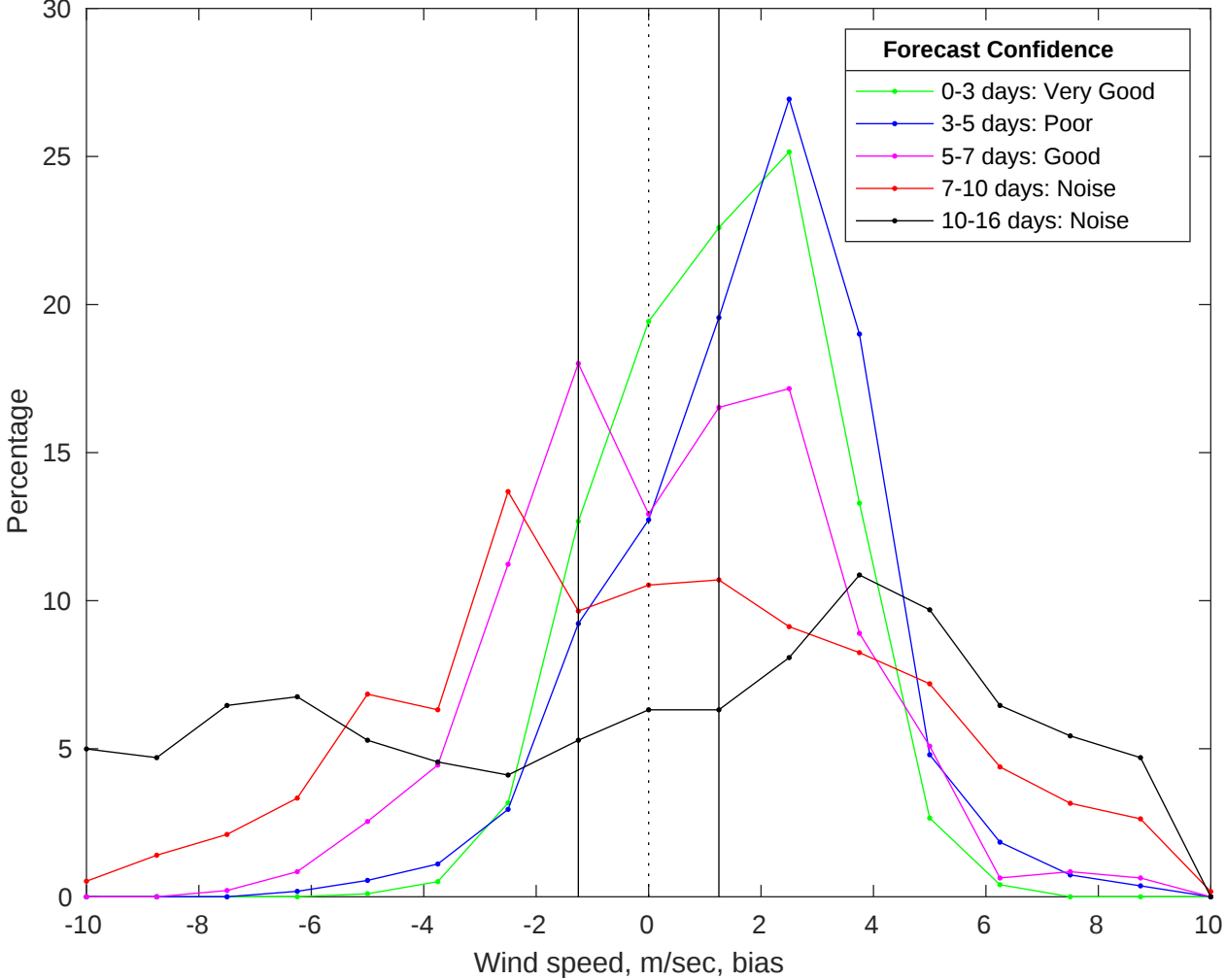
NDBC 46028 vs GFS Winds Bias Histogram: 16-Jun-2025
