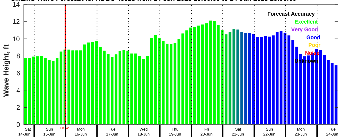
CMEMS Wave Forecast for NDBC 46028 from 14-Jun-2025 16:00:00 to 24-Jun-2025 16:00:00
