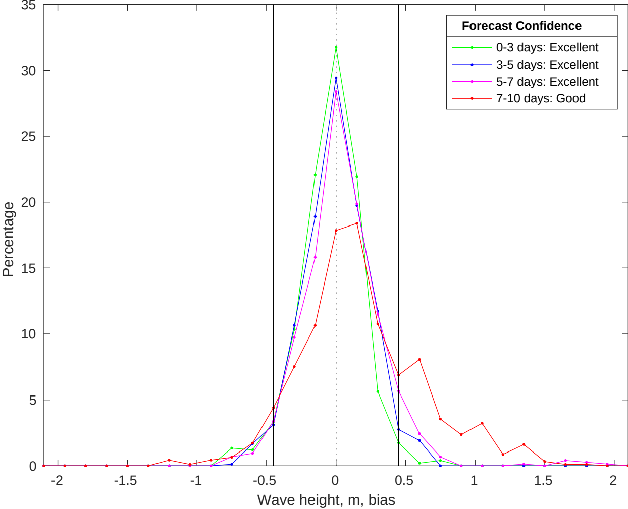
NDBC 46054 vs CMEMS Waves Bias Histogram: 16-Jun-2025
