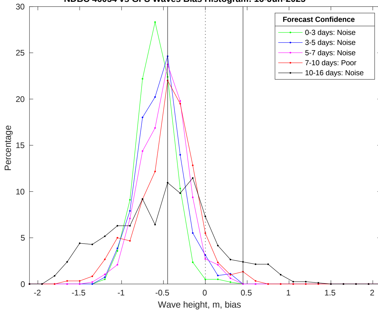
NDBC 46054 vs GFS Waves Bias Histogram: 16-Jun-2025
