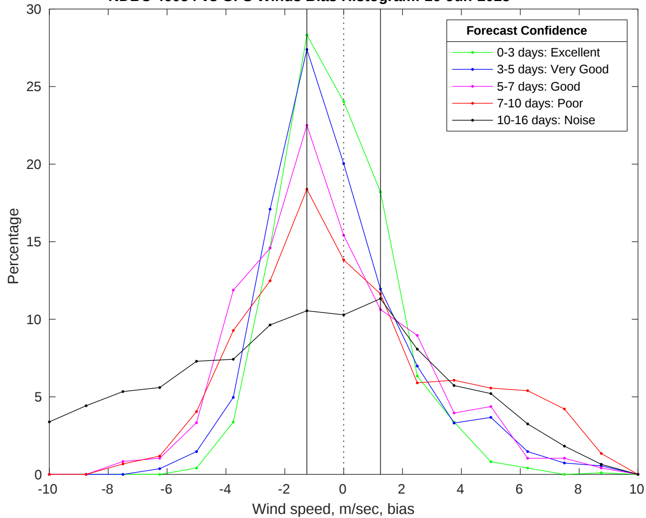
NDBC 46054 vs GFS Winds Bias Histogram: 16-Jun-2025
