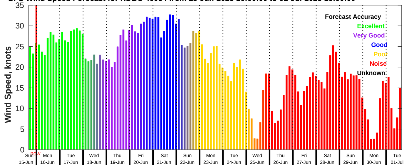
GFS Wind Speed Forecast for NDBC 46054 from 15-Jun-2025 16:00:00 to 01-Jul-2025 16:00:00
