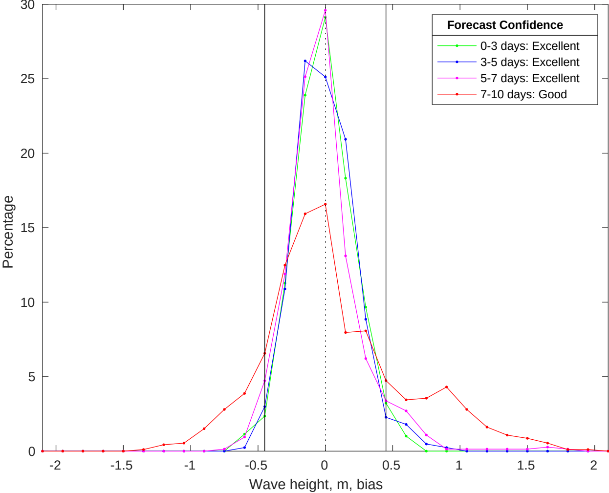
NDBC 46069 vs CMEMS Waves Bias Histogram: 16-Jun-2025
