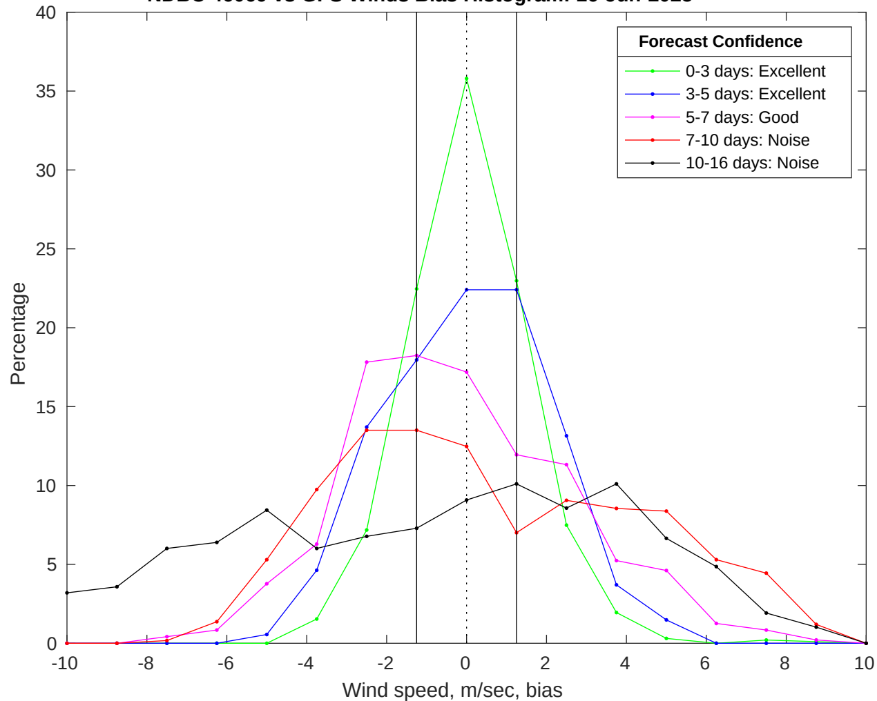
NDBC 46069 vs GFS Winds Bias Histogram: 16-Jun-2025
