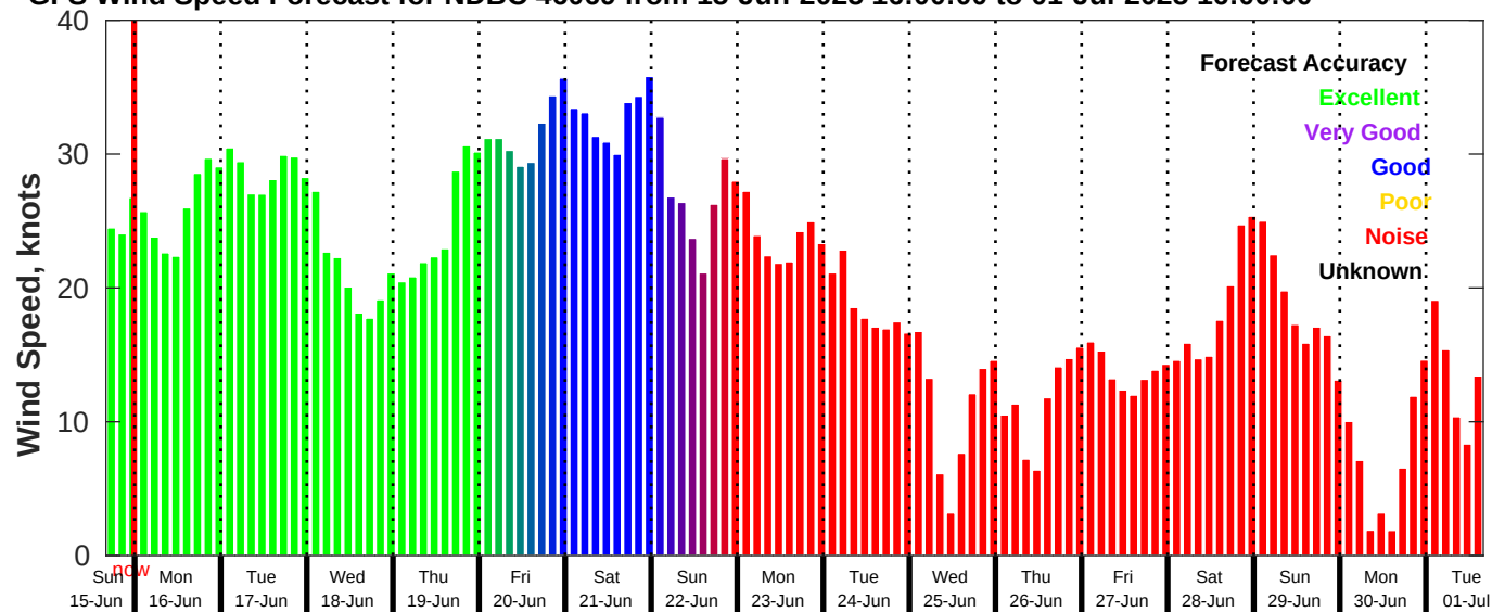
GFS Wind Speed Forecast for NDBC 46069 from 15-Jun-2025 16:00:00 to 01-Jul-2025 16:00:00
