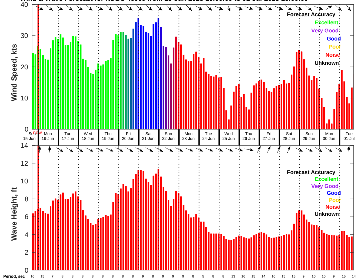
Wind & Wave Forecast for NDBC 46069 from 15-Jun-2025 16:00:00 to 01-Jul-2025 16:00:00
