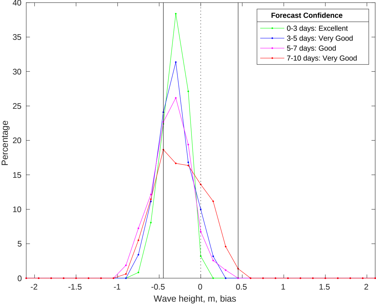
NDBC 51209 vs CMEMS Waves Bias Histogram: 16-Jun-2025
