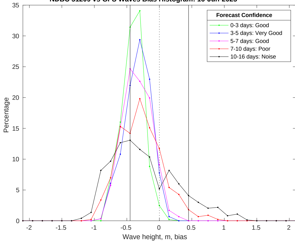
NDBC 51209 vs GFS Waves Bias Histogram: 16-Jun-2025
