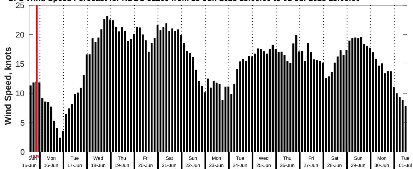
GFS Wind Speed Forecast for NDBC 51209 from 15-Jun-2025 13:00:00 to 01-Jul-2025 13:00:00
