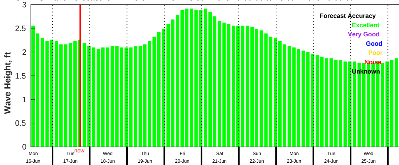
CMEMS Wave Forecast for NDBC 52211 from 15-Jun-2025 10:00:00 to 25-Jun-2025 10:00:00
