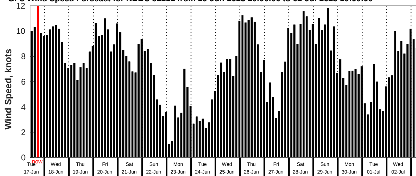
GFS Wind Speed Forecast for NDBC 52211 from 16-Jun-2025 10:00:00 to 02-Jul-2025 10:00:00
