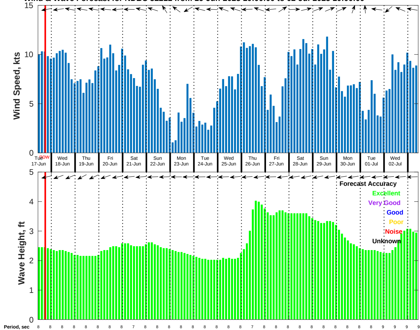
Wind & Wave Forecast for NDBC 52211 from 16-Jun-2025 10:00:00 to 02-Jul-2025 10:00:00
