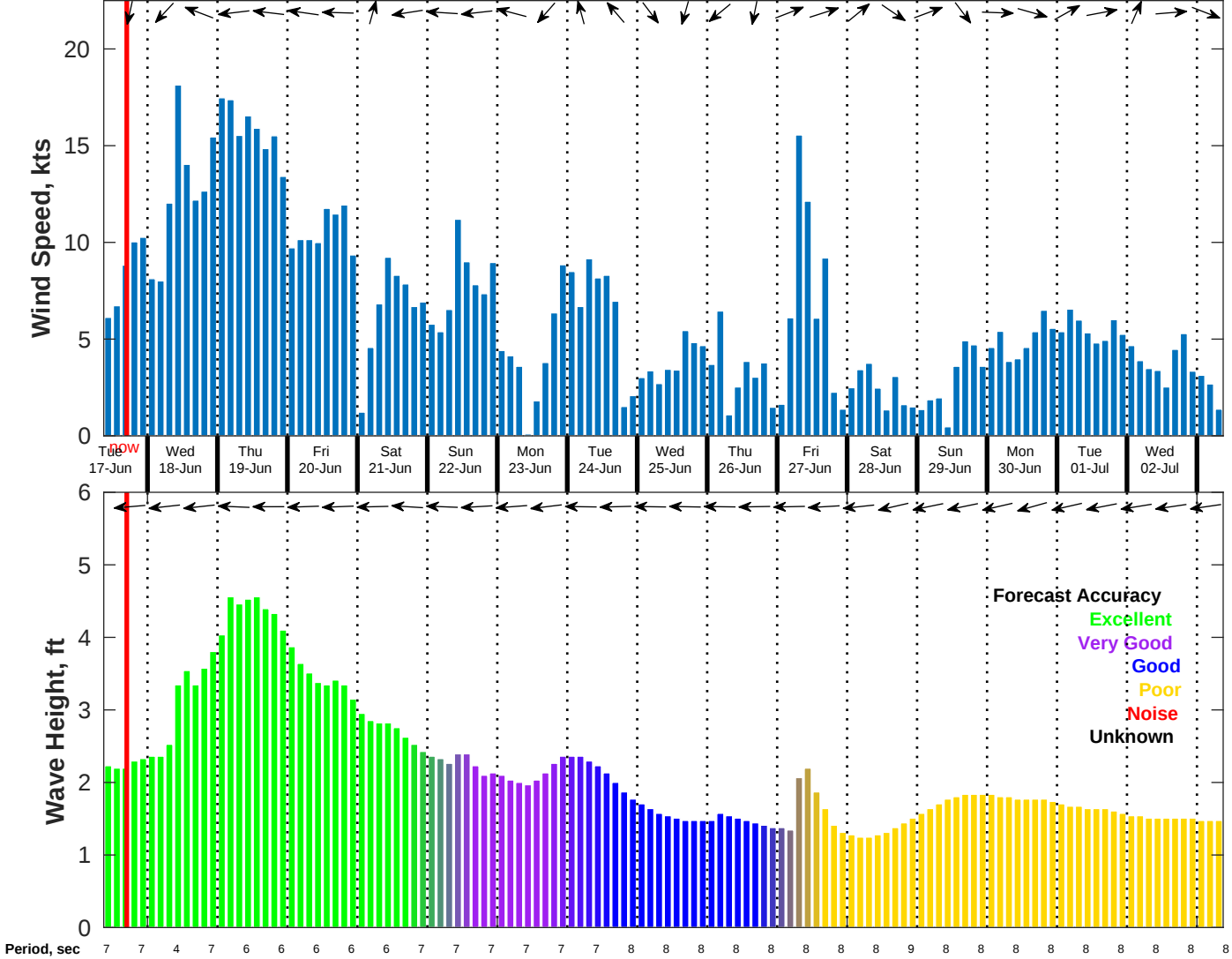
Wind & Wave Forecast for NDBC 52212 from 16-Jun-2025 09:00:00 to 02-Jul-2025 09:00:00
