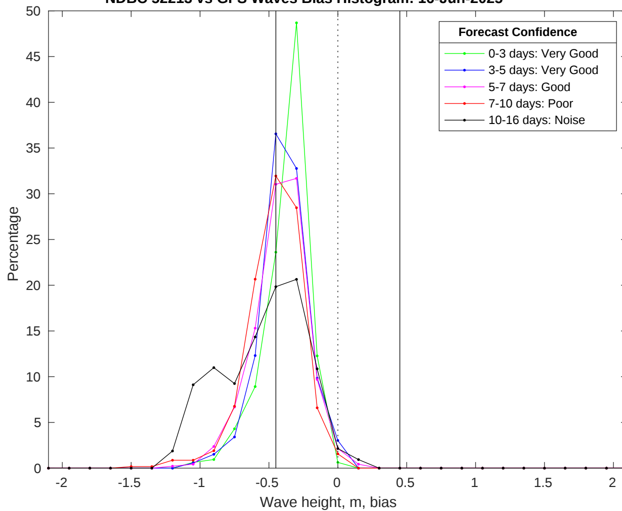
NDBC 52213 vs GFS Waves Bias Histogram: 16-Jun-2025
