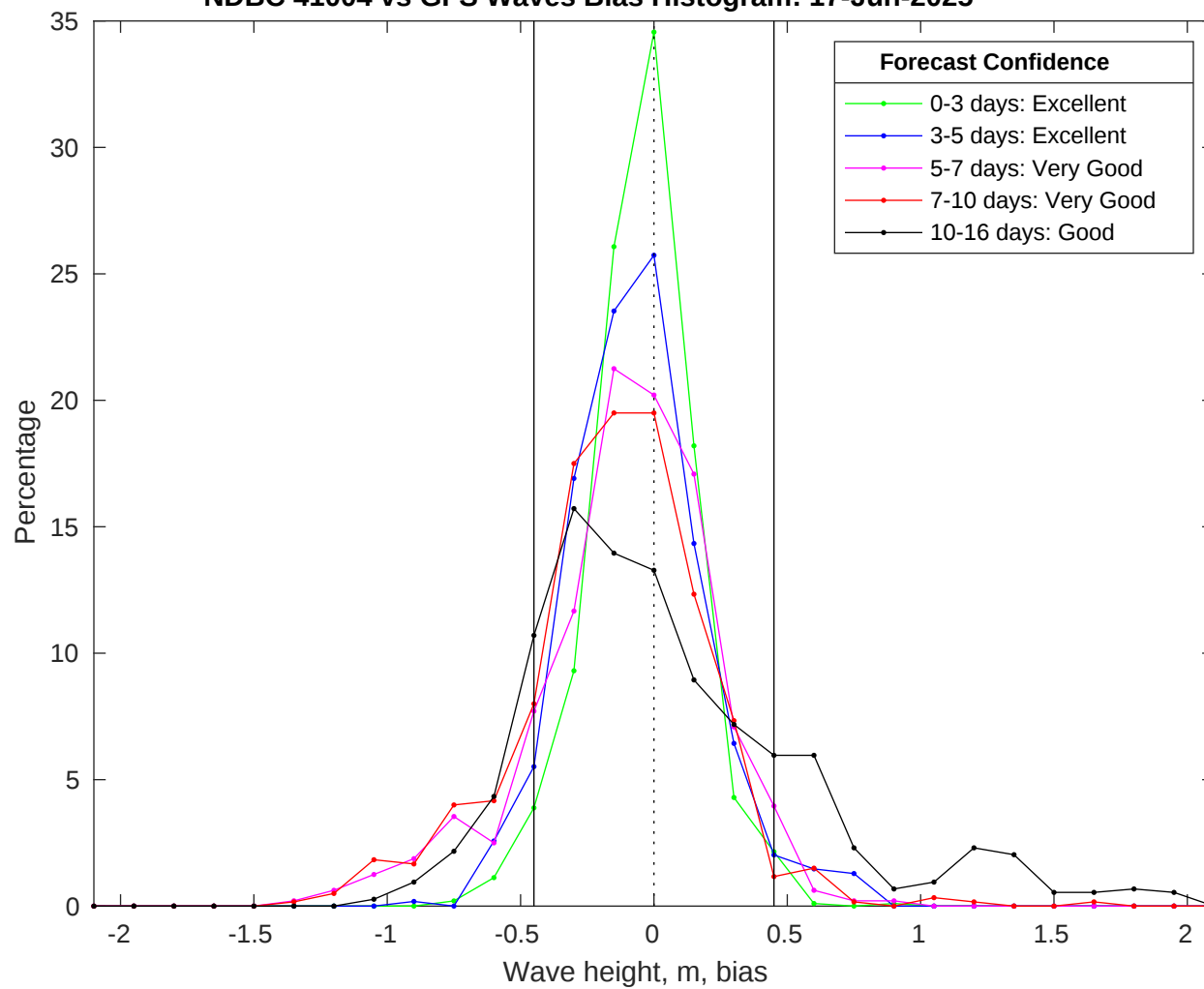
NDBC 41004 vs GFS Waves Bias Histogram: 17-Jun-2025
