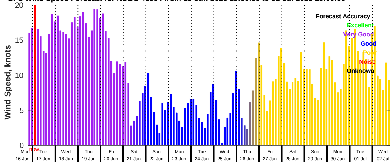
GFS Wind Speed Forecast for NDBC 41004 from 16-Jun-2025 19:00:00 to 02-Jul-2025 19:00:00
