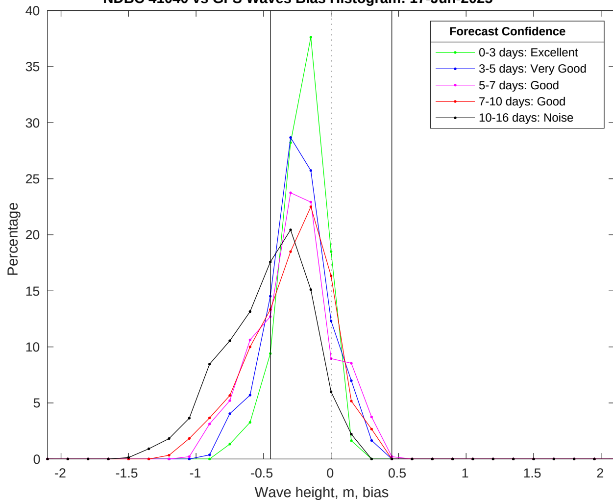
NDBC 41040 vs GFS Waves Bias Histogram: 17-Jun-2025
