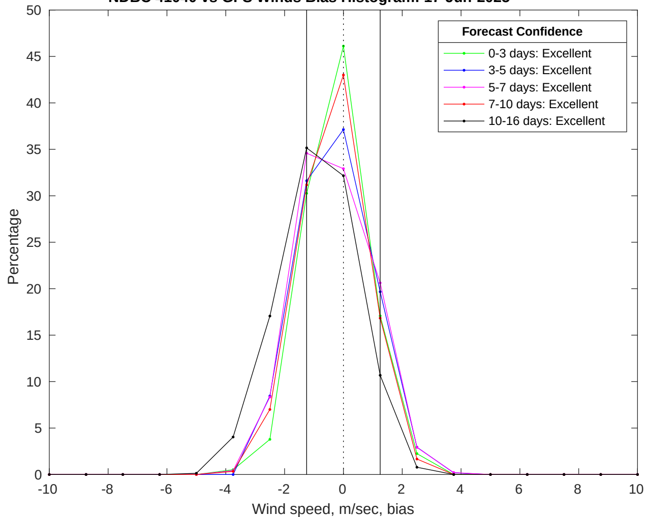
NDBC 41040 vs GFS Winds Bias Histogram: 17-Jun-2025
